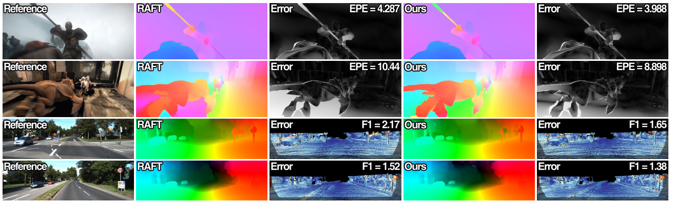
Figure 4: Qualitative comparisons with RAFT (?) on Sintel and KITTI test set. All results are provided by the official website of each dataset. Best viewed in color.
